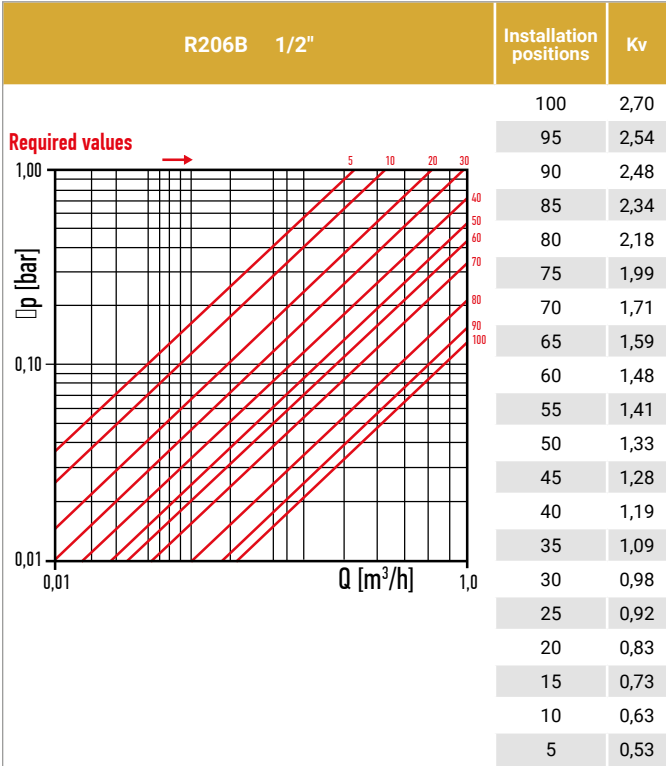
Diagram of pressure losses vs. flow rate for a partner valve
