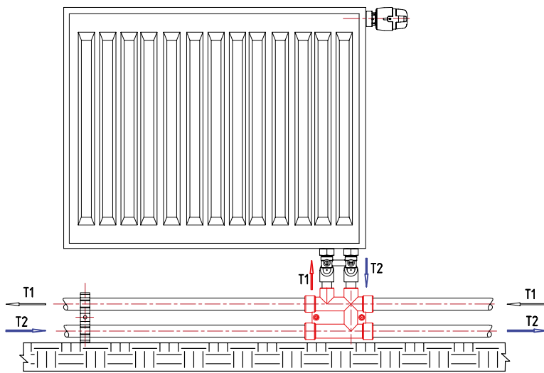
PANEL RADIATOR
