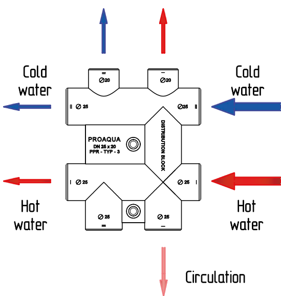
WATER SUPPLY
